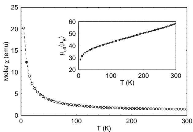
Figure 4. \chi (emu/mole) vs T plot at 100 G. Dashed line is a guide to the eye. Inset shows the effective magnetic moment ( \mu_{\text{eff}} ) as a function of T .
