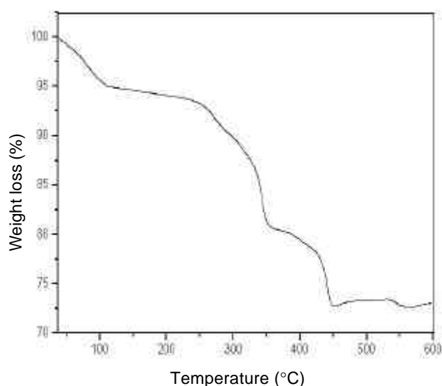
Figure 1. Thermogravimetric analysis (TGA) of I .
