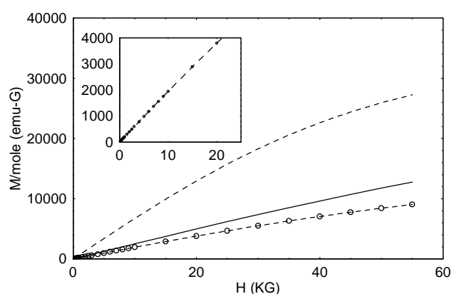
Figure 5. Magnetization ( M ) as a function of field ( H ) at 5.5 K (circles). Theoretically calculated M(H) for a unit spin of S = 9 (solid line) and for 18 independent S = 1/2 spins (dashed line) are also shown. Note that the experimental M(H) is close to that for a unit spin of S = 9 . Inset shows the initial rapid rise of the M (see text).
