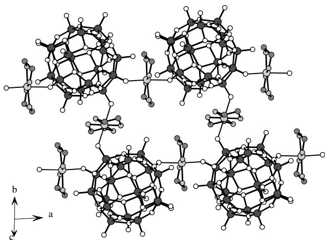
Figure 3. [\text{Zn}_2(\text{en})_5][\{\text{Zn}(\text{en})_2\}_2\{\text{V}_{18}\text{O}_{42}(\text{H}_2\text{O})\}]\cdot x\text{H}_2\text{O} ( x \sim 12 ), I , showing the connectivity between the \text{V}_{18}\text{O}_{42} clusters. Hydrogen atoms of the amine molecule are not shown for clarity. The layers are separated by another Zn-ethylenediamine complex (not shown).
