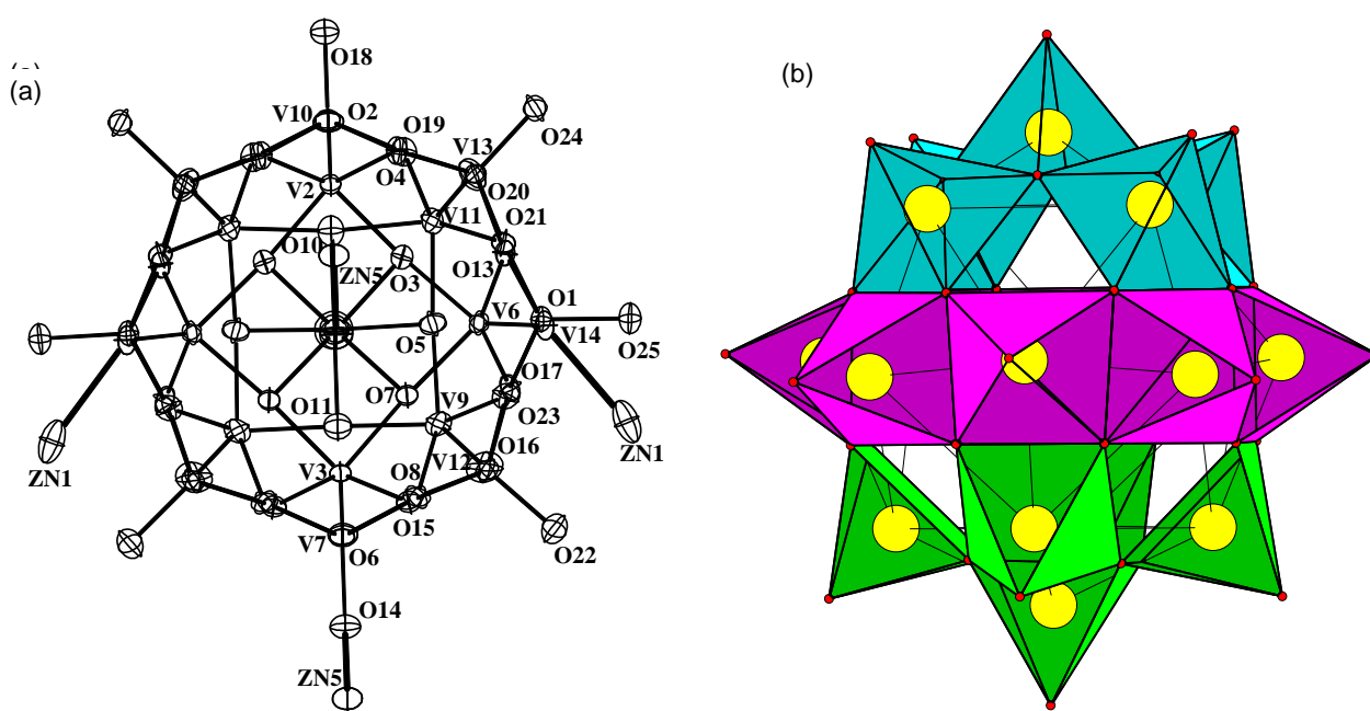
Figure 2. (a) Single [V_{18}O_{42}]^{12-} cluster with the labeling. Thermal ellipsoids are given at 50% probability. (b) The polyhedral view of one single [V_{18}O_{42}]^{12-} cluster.
